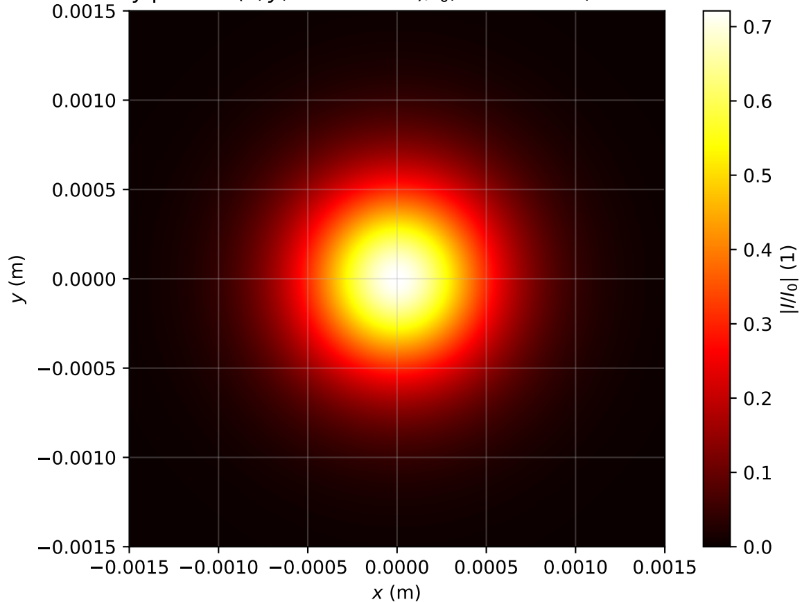
Intensity profile I(x, y, z = 3.503m)/I_0 , P_{in}=0.7P_{cr} , artificial time
